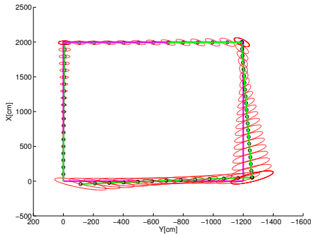
Figure 4. Estimated trajectory of the robot before applying the closing loop. Purple and green lines indicate true and estimated trajectories, respectively. Black circles indicate the estimated position where robot observed. Red ellipsoids indicate 99% probability ellipsoid of the robot position.
