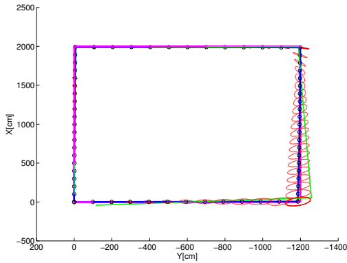
Figure 5. Estimated trajectory of the robot after applying the closing loop. Two trajectories (purple and green lines) are the same as Fig. 4. Blue line indicates the estimated trajectory after applying the closing loop. The estimated positions (black circle) and their 99% probability ellipsoids (red ellipsoid) are on the trajectory after applying the closing loop.
